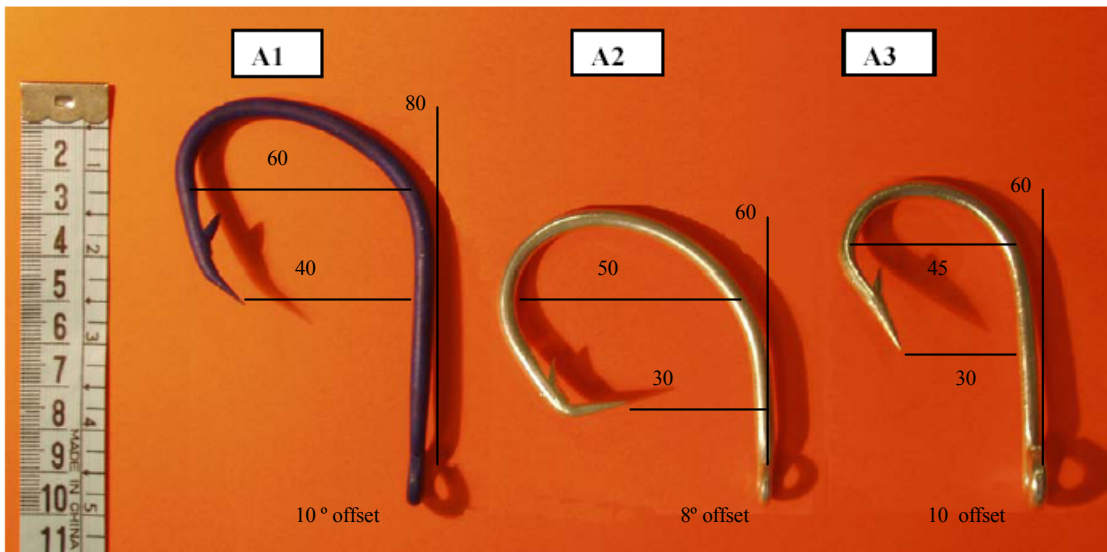
Figure 2. Three types of hooks tested during the survey, sizes (mm) and offset (degrees). A1 : the new semicircular “SG” hook 18/O (10° offset) = 80 – 60 – 40 and blue in colour (as proposed by the fleet itself). A2 : Circle “G” hook 17/O (8° offset) = 60 – 50 – 30. A3 : Conventional “J” hook 16/O (10° offset) “J” = 60 – 45 – 30.
