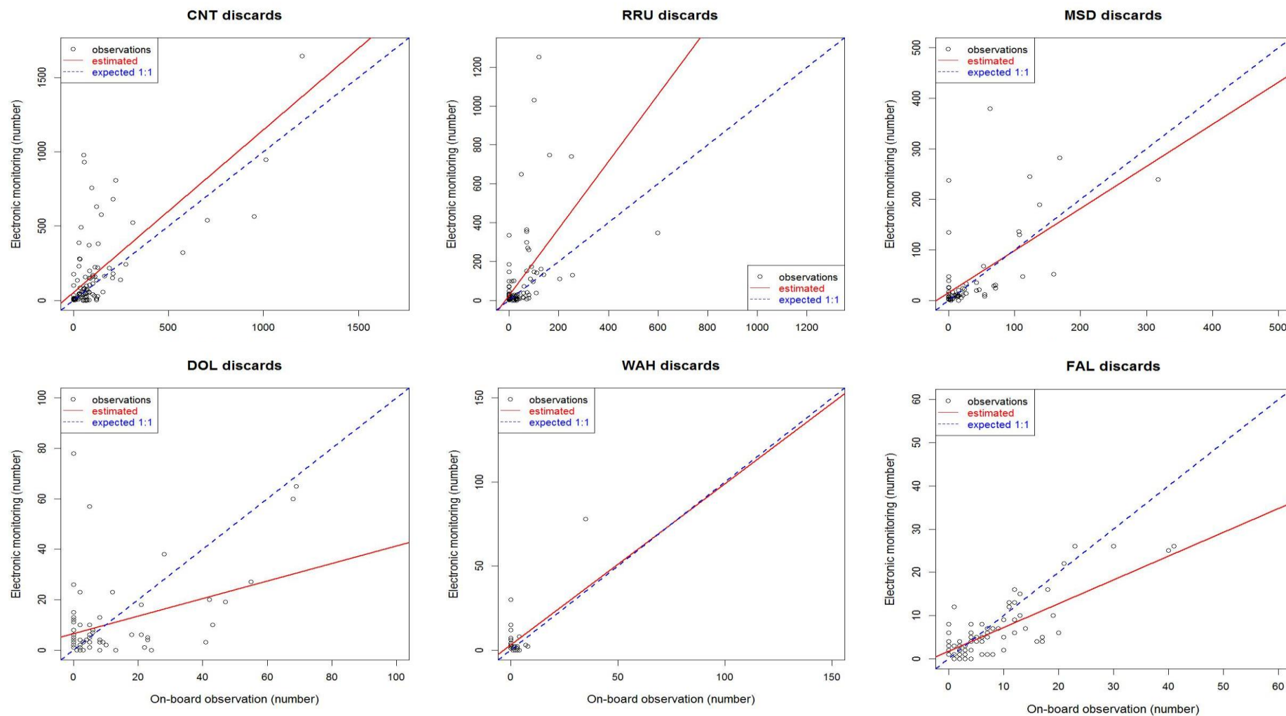
Figure 7. Estimated regression (solid line) and expected 1:1 relationship (dashed line) between EMS and on-board observers records of non-target catch discards. GLM analysis was performed for individual non-target species Canthidermis maculate CNT (N=99), Elegatis bipinnulata RRU (N=91), Decapterus macarellus MSD (N=66), Coryphaena hippurus DOL (N=77), Acanthocybium solandri WAH (N=41) and Carcharhinus falciformis FAL (N=88).
