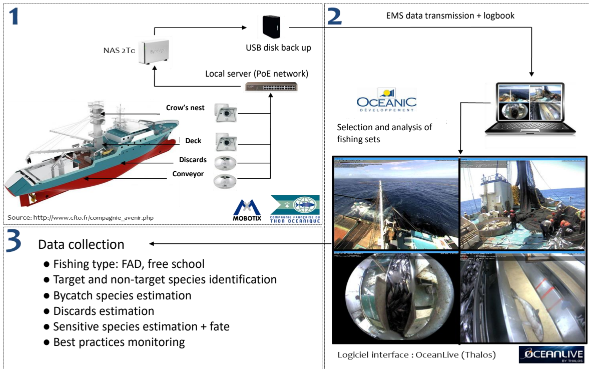
Figure 2. Schematic representation of the EMS installation and the process of data.
