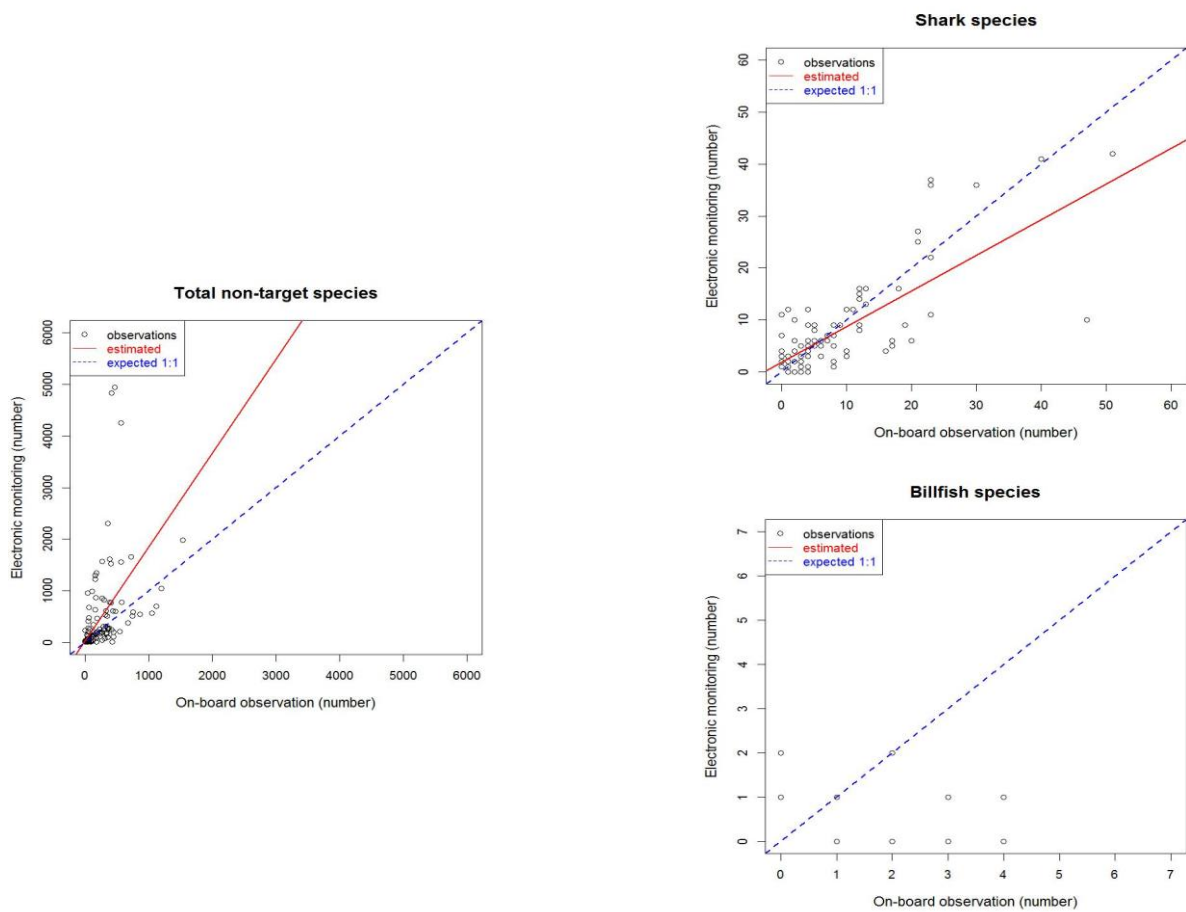
Figure 4. Estimated regression (solid line) and expected 1:1 relationship (dashed line) between EMS and on-board observers records of non-target catch. GLM analysis was performed for total non-target species (N=124) and for sharks (N=105) and billfishes (N=36) species.
