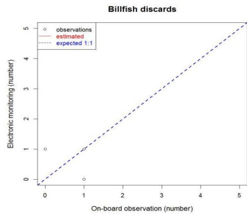
Figure 6. Estimated regression (solid line) and expected 1:1 relationship (dashed line) between EMS and on-board observers records of non-target catch discards. GLM analysis was performed for total non-target catch discards (N=109) and for sharks (N=92) and billfishes discards (N=11).
