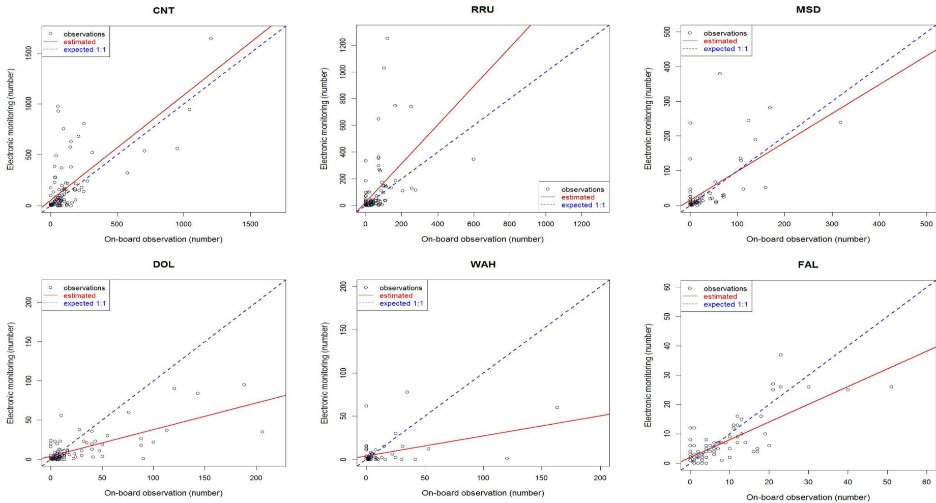
Figure 5. Estimated regression (solid line) and expected 1:1 relationship (dashed line) between EMS and on-board observers records of non-target catch. GLM analysis was performed for individual non-target species Canthidermis maculate CNT (N=100), Elegatis bipinnulata RRU (N=96), Decapterus macarellus MSD (N=66), Coryphaena hippurus DOL (N=93), Acanthocybium solandri WAH (N=69) and Carcharhinus falciformis FAL (N=96).
