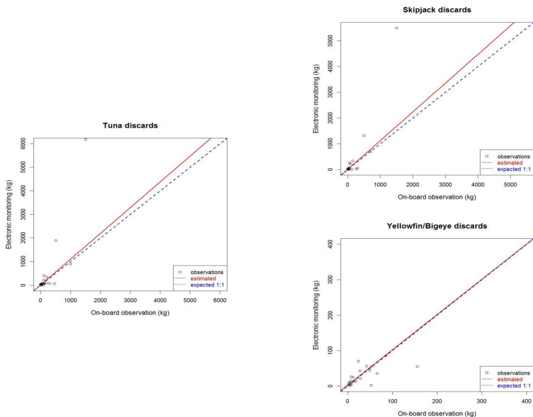
Figure 3. Estimated regression (solid line) and expected 1:1 relationship (dashed line) between EMS and on-board observers records of tuna discards. GLM analysis was performed for total tuna discards (N=42) and for skipjack (N=33) and yellowfin/bigeye (N=23) tuna discards.
